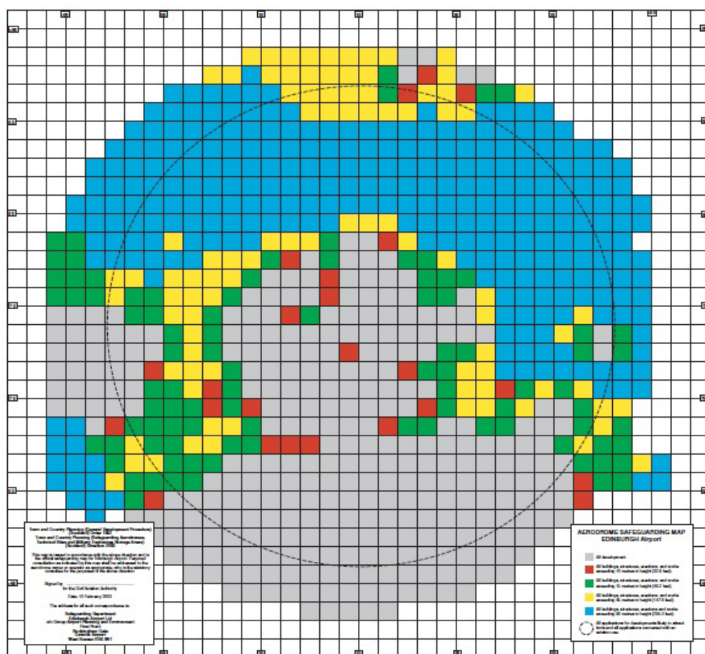
Example Safeguarding Map – extending out to 15km from the runway (aerodrome reference point), also depicting a 13km dotted circle and grid legend
